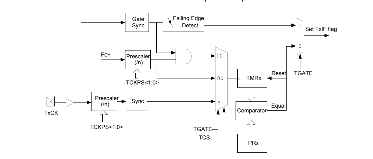
FIGURE 13-1: TYPE B TIMER BLOCK DIAGRAM (x = 2 or 4)
