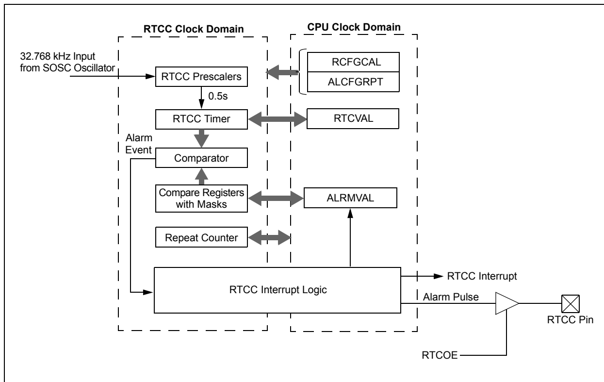
FIGURE 25-1: RTCC BLOCK DIAGRAM
