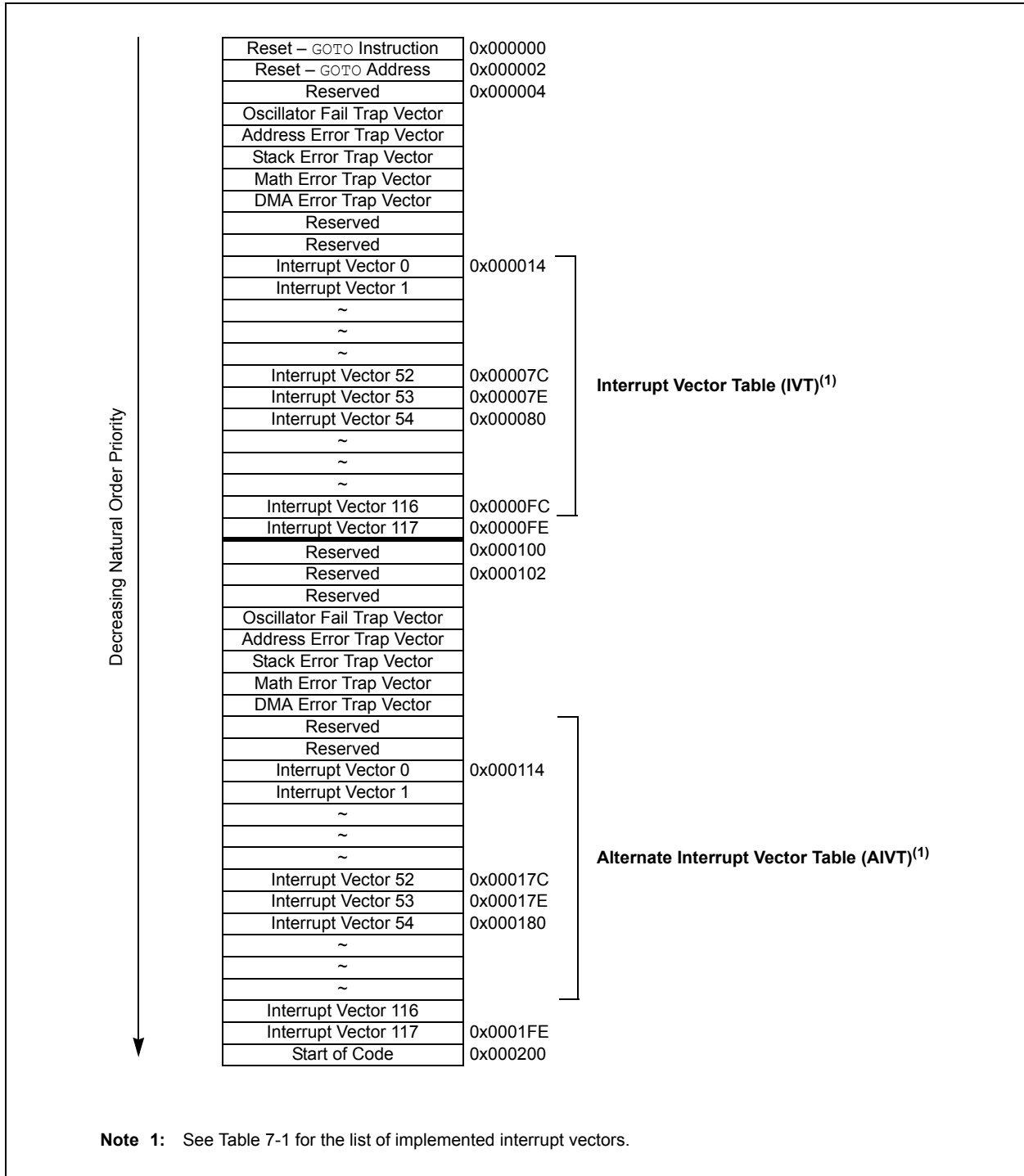
FIGURE 7-1: dsPIC33FJ32MC302/304, dsPIC33FJ64MCX02/X04, AND dsPIC33FJ128MCX02/X04 INTERRUPT VECTOR TABLE
