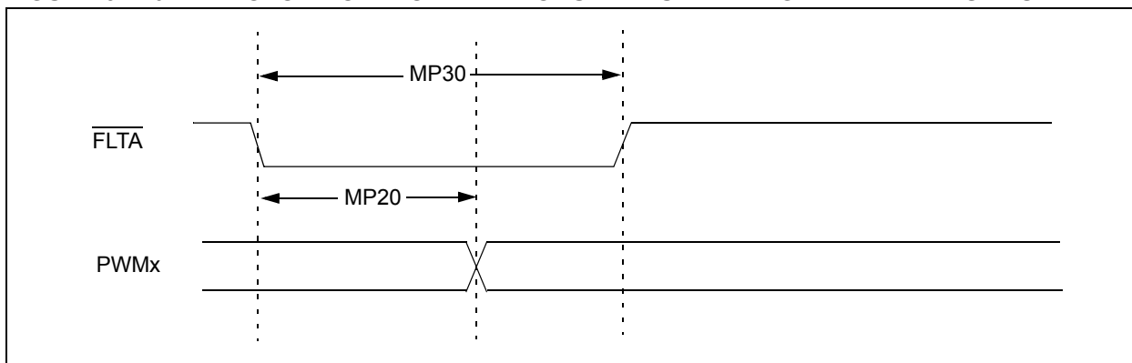
FIGURE 31-10: MOTOR CONTROL PWM MODULE FAULT TIMING CHARACTERISTICS
