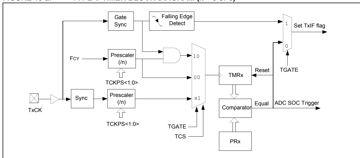
FIGURE 13-2: TYPE C TIMER BLOCK DIAGRAM (x = 3 or 5)
