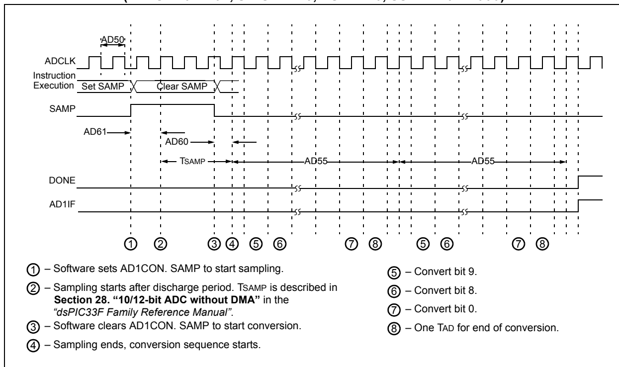
FIGURE 31-24: ADC CONVERSION (10-BIT MODE) TIMING CHARACTERISTICS (CHPS<1:0> = 01, SIMSAM = 0, ASAM = 0, SSRC<2:0> = 000)
